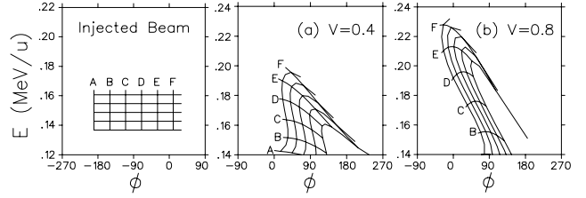
Fig. 116. Final positions in E - \phi space of initial grid of particles after acceleration through tank 1 for voltages of 40% and 80% of the full energy setting.
