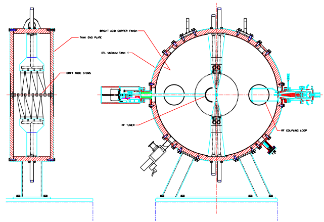
Fig. 119. The DTL buncher, side and end views. The side view shows the attached diagnostic box.
