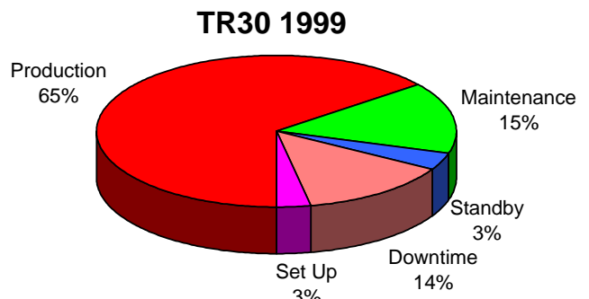
Fig. 177. Breakdown of downtime and maintenance for the CP42 (top) and TR30 (bottom) during operational hours.
