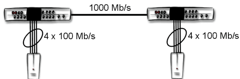
Figure 3. Switch-to-station connection
