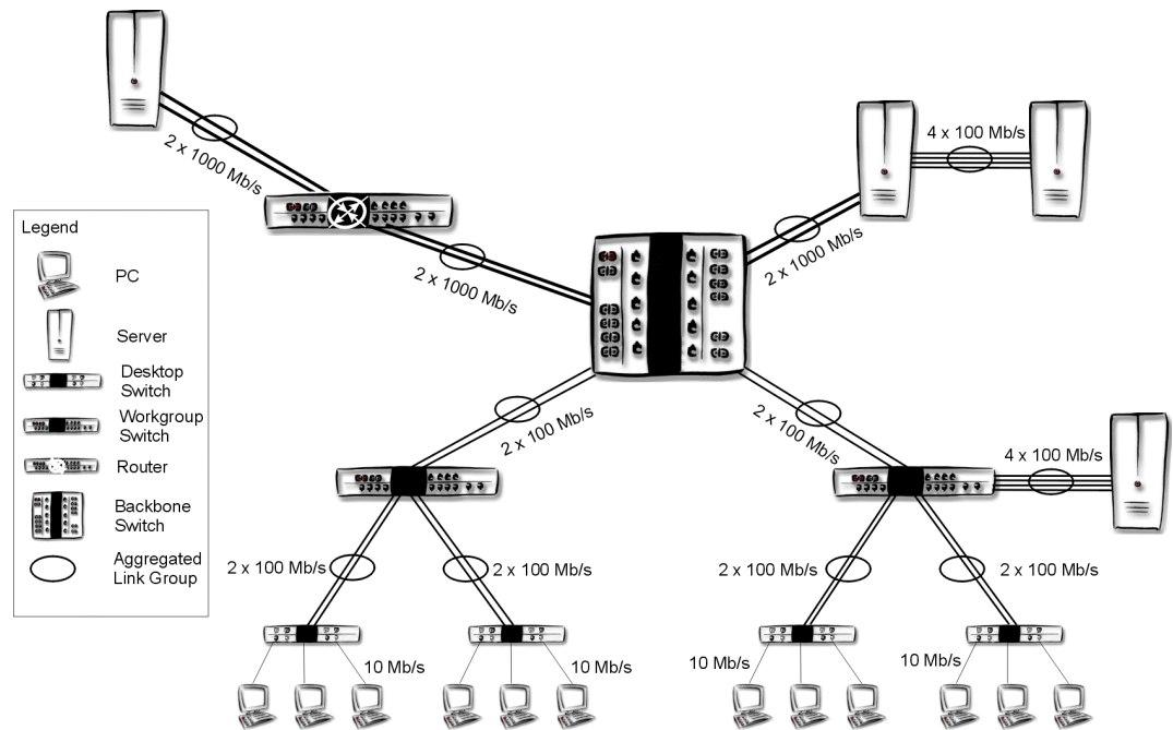
Figure 1. Aggregated links
