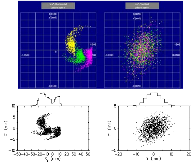
Figure 2: Comparison of Agile (top) and Accsim phase-space plots (the closed orbit deviation is removed in the Accsim plot).
