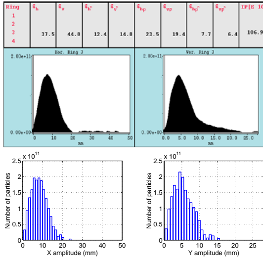
Figure 1: Comparison of BeamScope (top) and Accsim profiles
